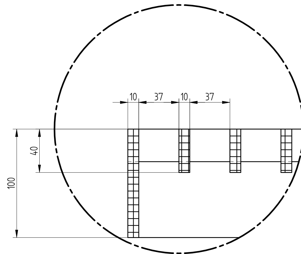
DETAIL B
